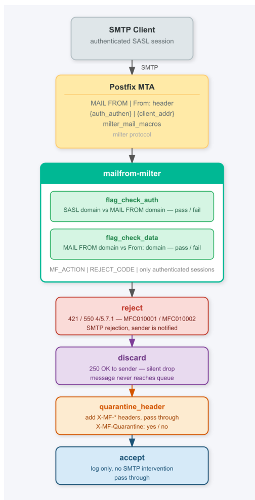
Figure 1: mailfrom-milter architecture
