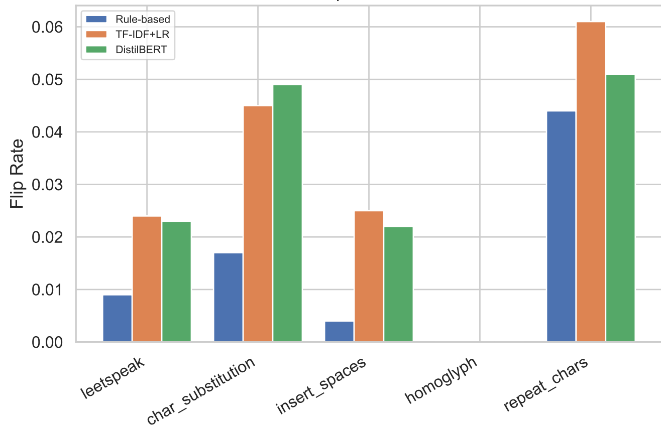
Prediction Flip Rate Under Attacks
