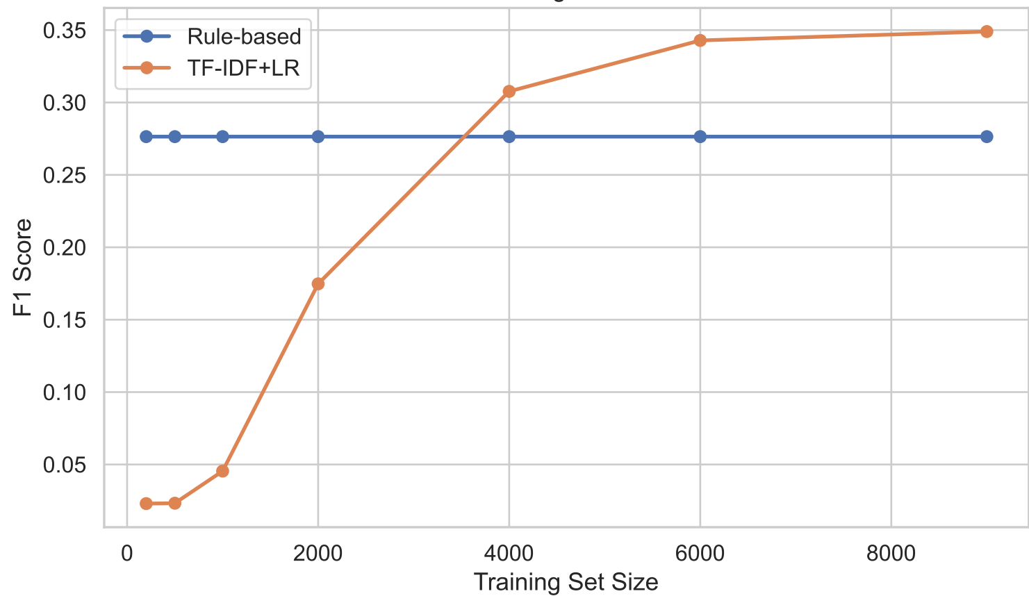
Effect of Training Data Size on F1
