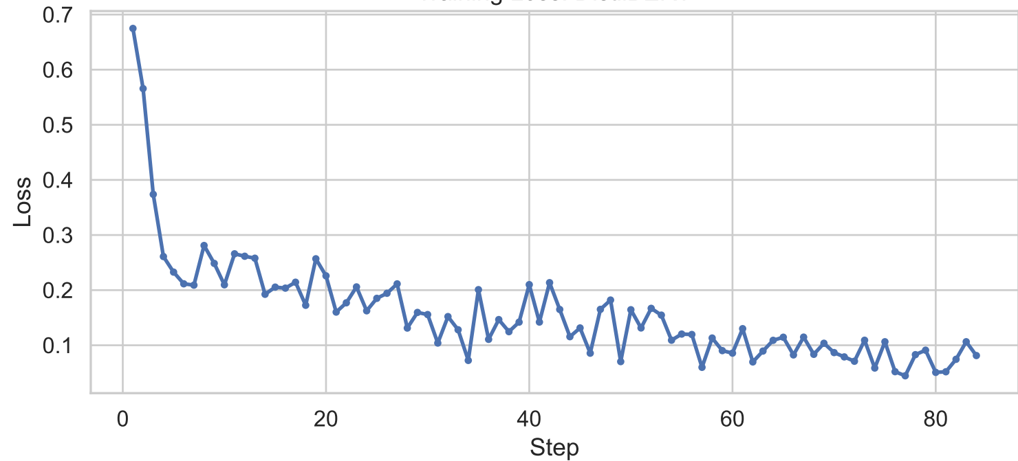
Training Loss: DistilBERT
