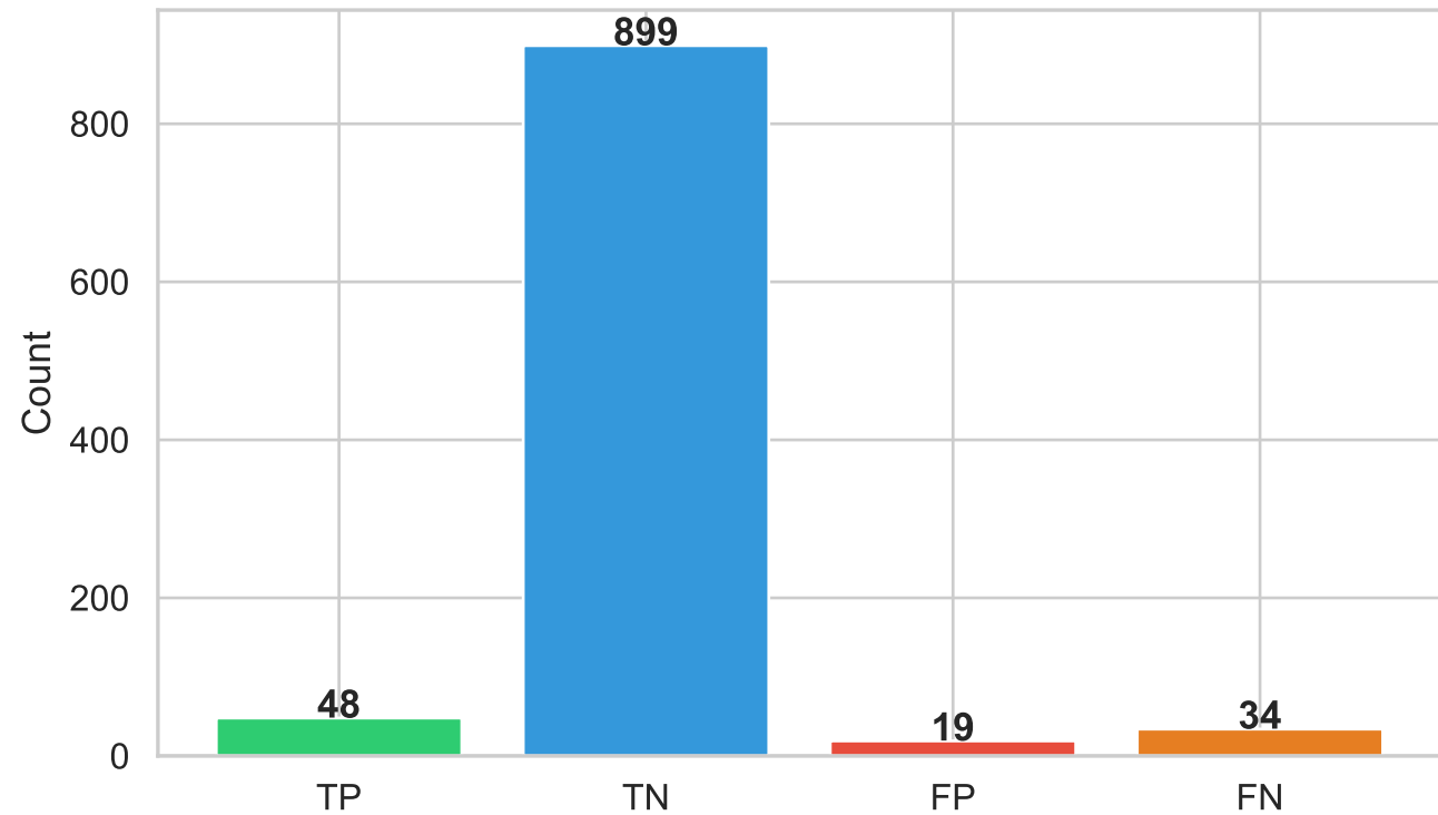
Prediction Breakdown
