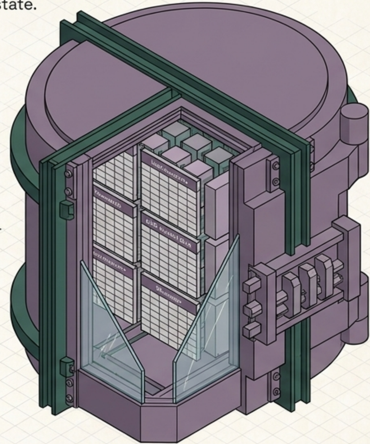
Persistent Database
