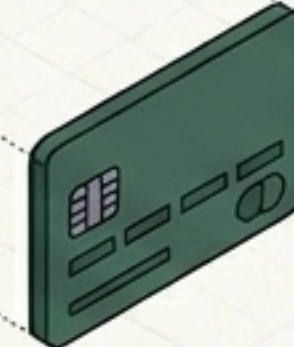
Payment API
