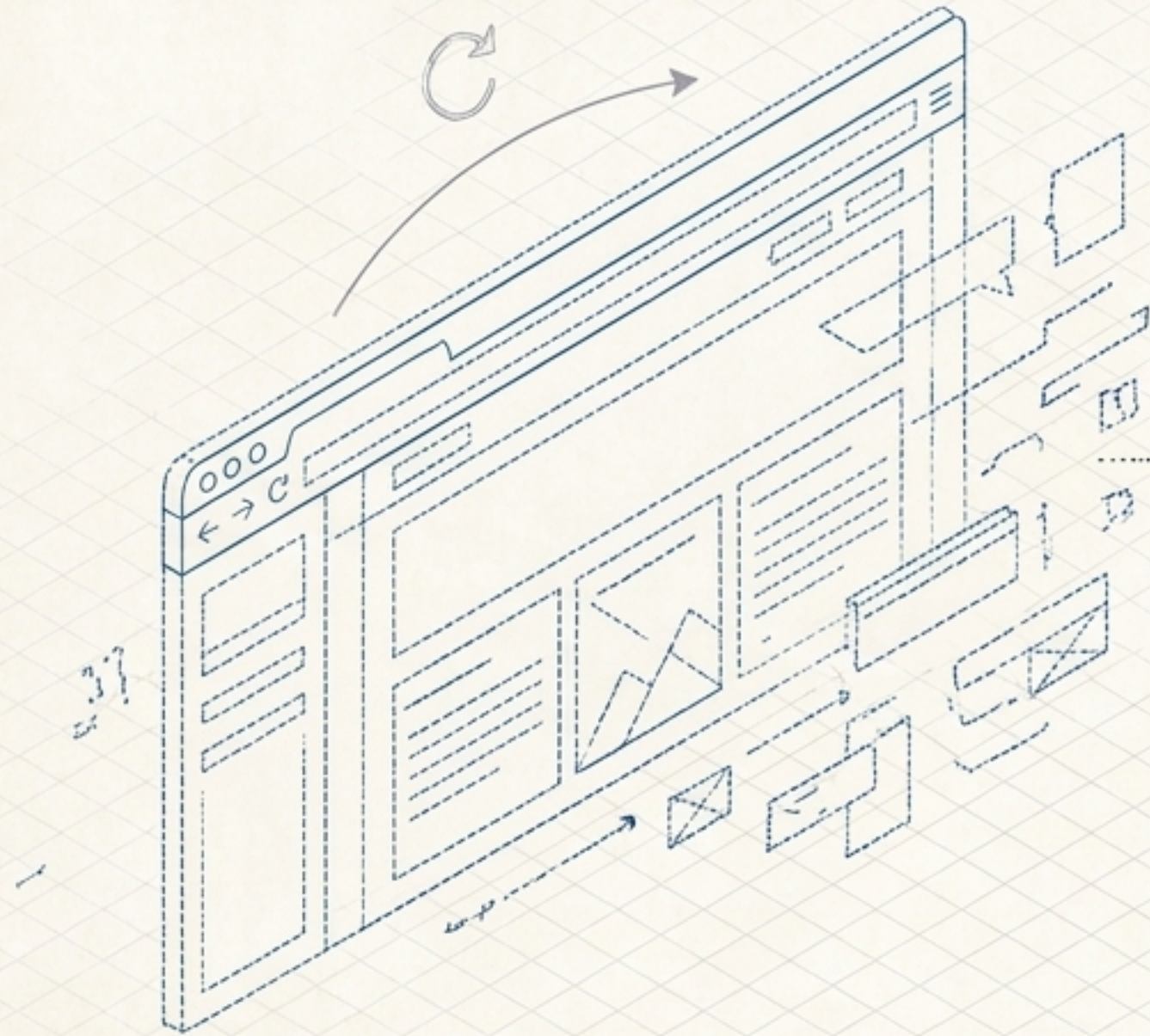
Volatile Memory
