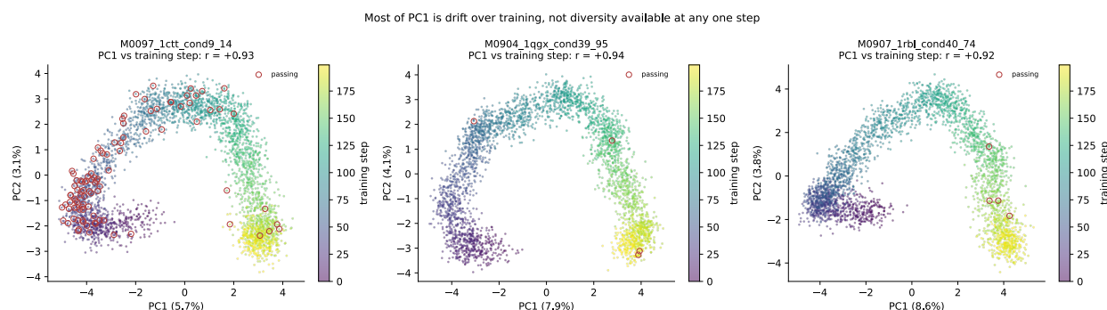
Figure 2: Most of PC1 is drift over training, not diversity available at any one step. The full GRPO trajectory for each backbone, in the same projection as Figure 1, coloured by training step; passing designs are circled. PC1 correlates with training step at r = +0.92 to +0.94 on all three backbones. This distinction is load-bearing rather than cosmetic: spread accumulated by drifting across training is genuine library diversity when the library is assembled from the whole run, which is how ours is assembled, but it is not evidence that any single policy is diverse. Presenting the pooled projection alone would conflate the two and overstate the result, so the axis is shown rather than hidden.
