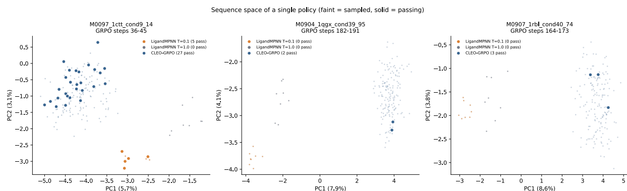
Figure 1: Sequence space occupied by each design method on the AME pilot backbones. One PCA per backbone, fit on every sequence that backbone contributes across all three arms, so the arms share one projection and the clouds are directly comparable. Faint points are sampled designs, solid points are designs that pass the benchmark criterion (motif all-atom RMSD < 1.5 \text{ \AA} , no ligand clash). CLEO is restricted to its peak-performing 10-step window so that three policies are compared at one point in training. On M0097 the low-temperature arm (orange) forms a tight knot displaced far along PC1 — five passing designs that are a single cluster at every identity threshold down to 50 % — while CLEO’s passing designs are spread throughout a broad cloud. T=1.0 (grey) reaches comparable spread with zero passing designs. Projections are deliberately not shared across backbones: a global fit places 99 % of PC1 variance on backbone identity, collapsing each backbone to its own blob and hiding the arm differences entirely. Explained variance is low (PC1 5 % to 9 %), as expected for one-hot encoded protein sequence; the projection is a visual aid and every quantitative claim in the text uses Hamming distance and cluster counts directly. Baseline arms hold 8 sequences each, so part of their compactness is small- n .
