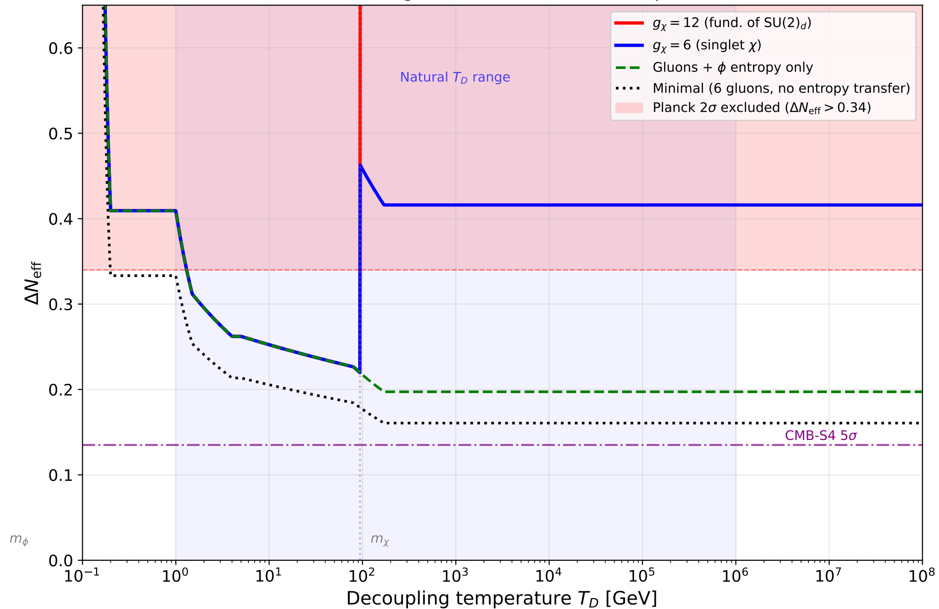
\Delta N_{\text{eff}} from dark gluons — \text{SU}(2)_d structural prediction
