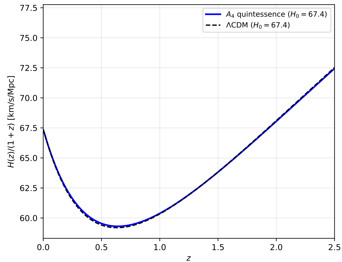
A_4 Quintessence: \Lambda_d = 1.40 meV, \theta_i = 1.57 rad, f = 4.5 M_{Pl}
