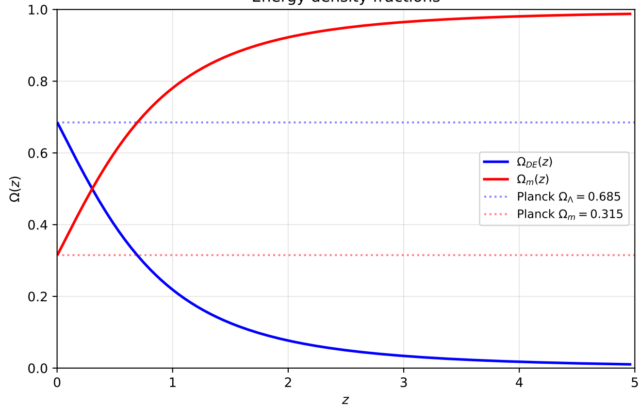
Energy density fractions
