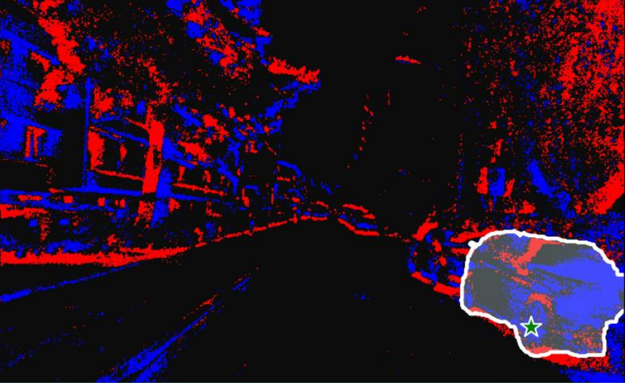
Car – Instance
