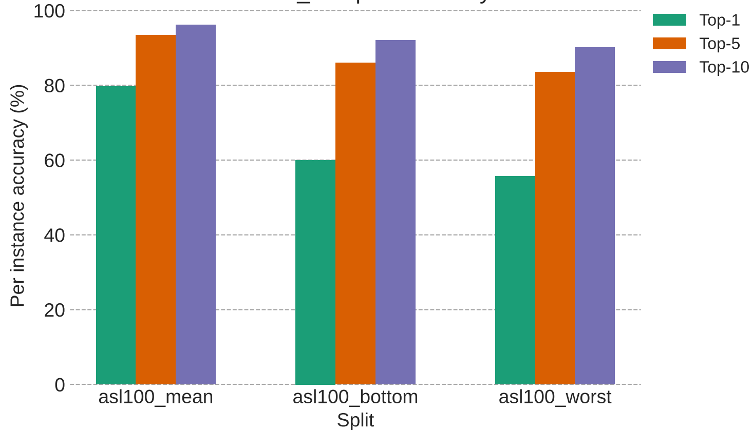
MViTv2_S Top-K Accuracy
