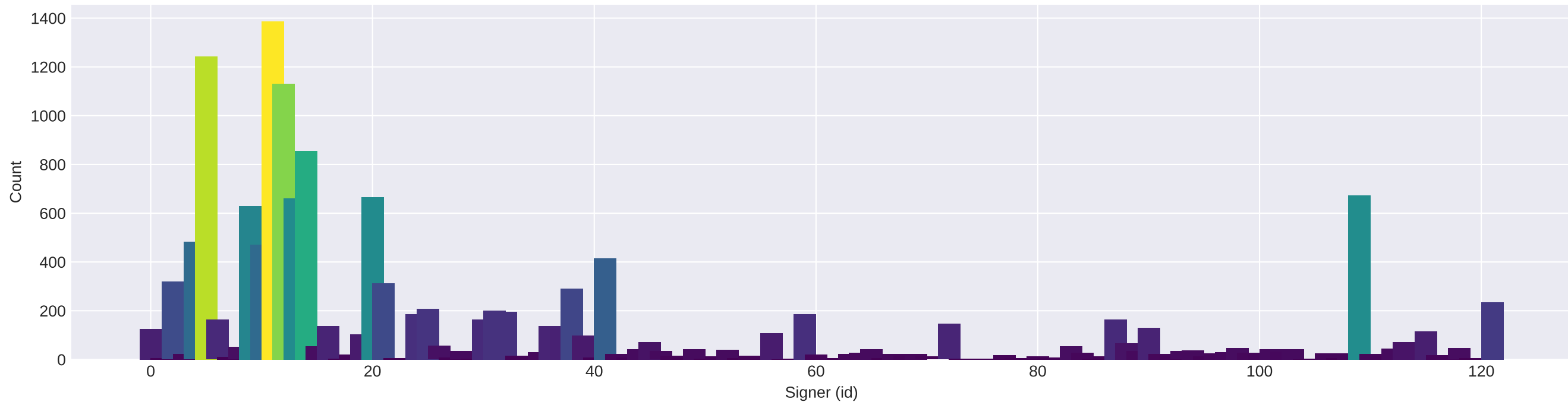
Signer Distribution: asl2000 / train
