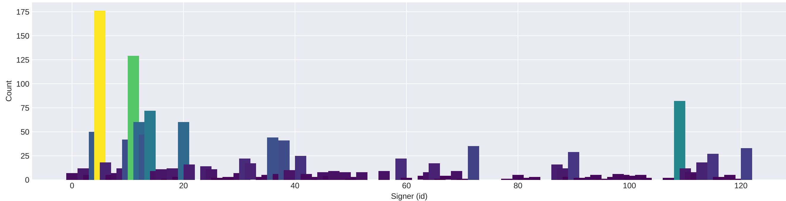
Signer Distribution: asl100 / train
