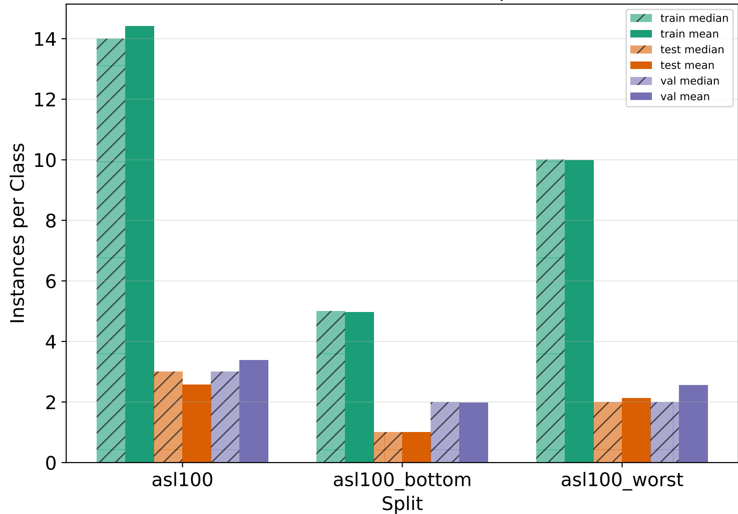
Mean & Median Instances per Class
