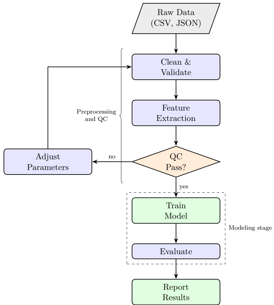
Figure 4.2: Vertical workflow diagram with preprocessing, quality control, and modeling stages.
