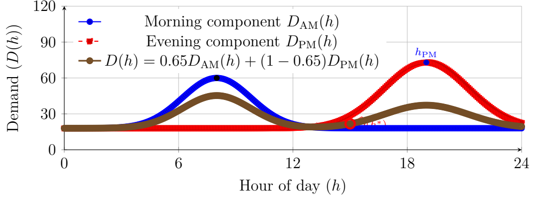
Figure 5.2: Dummy diurnal demand model. The solid curve shows a morning peak component, the dashed curve shows an evening peak component, and the thick curve shows their weighted blend. Markers indicate the component peak hours and a single-point prediction at h^* = 15 .
