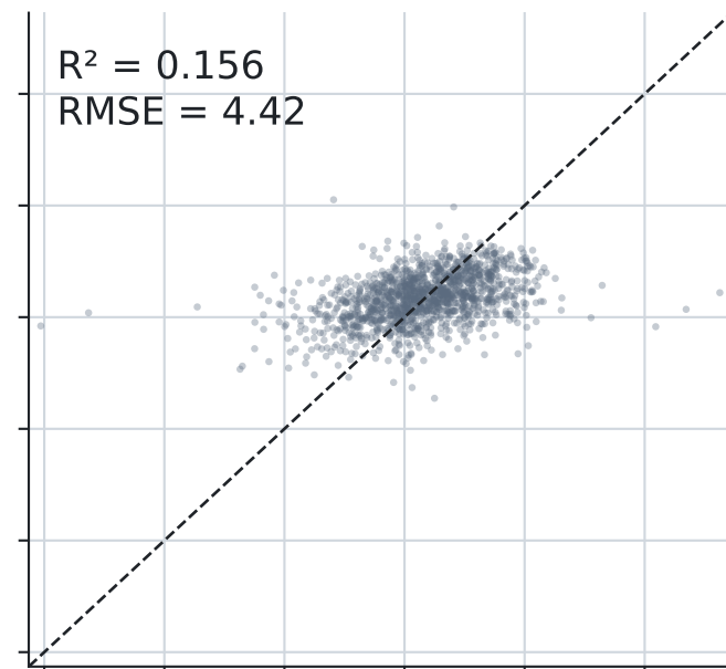
ChemBERTa-2
