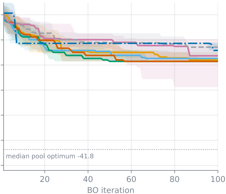
ChemBERTa-2
