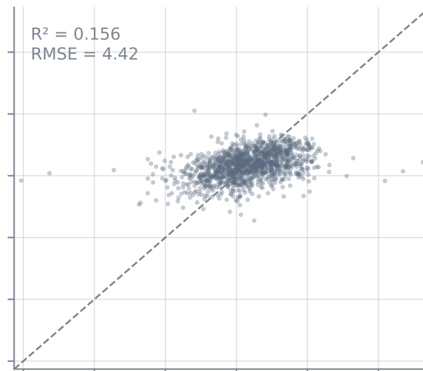
ChemBERTa-2
