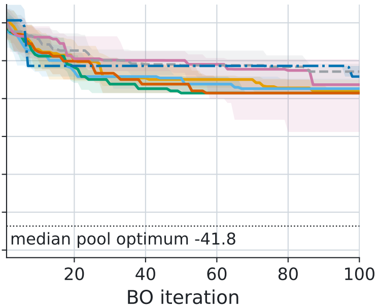
ChemBERTa-2
