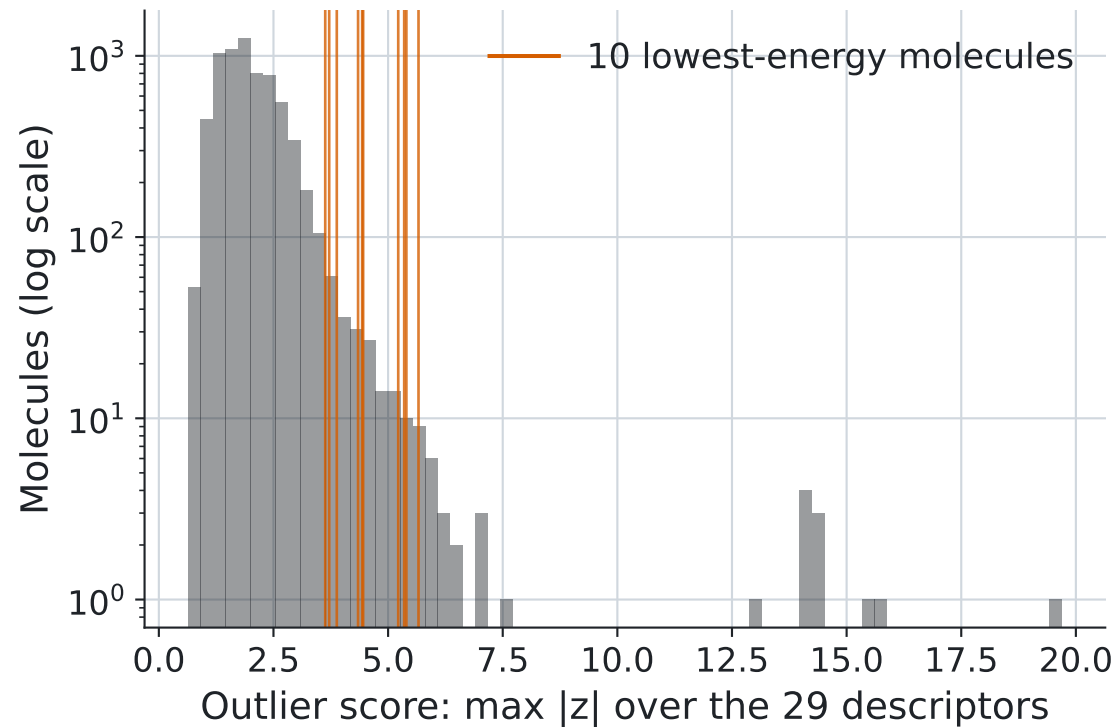
Outlier score distribution
