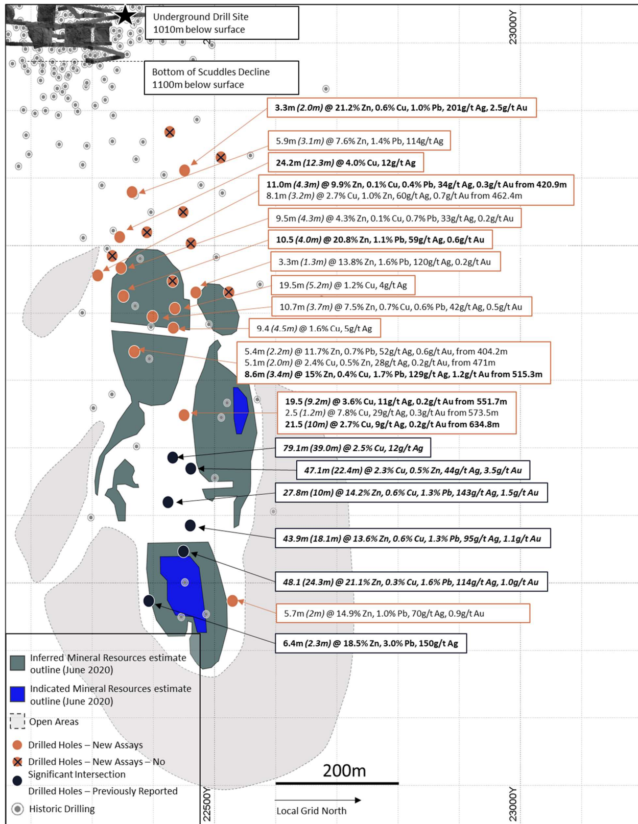
Figure 2 – Long section presentation of Cervantes
