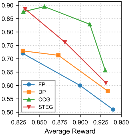
Safety Rate
