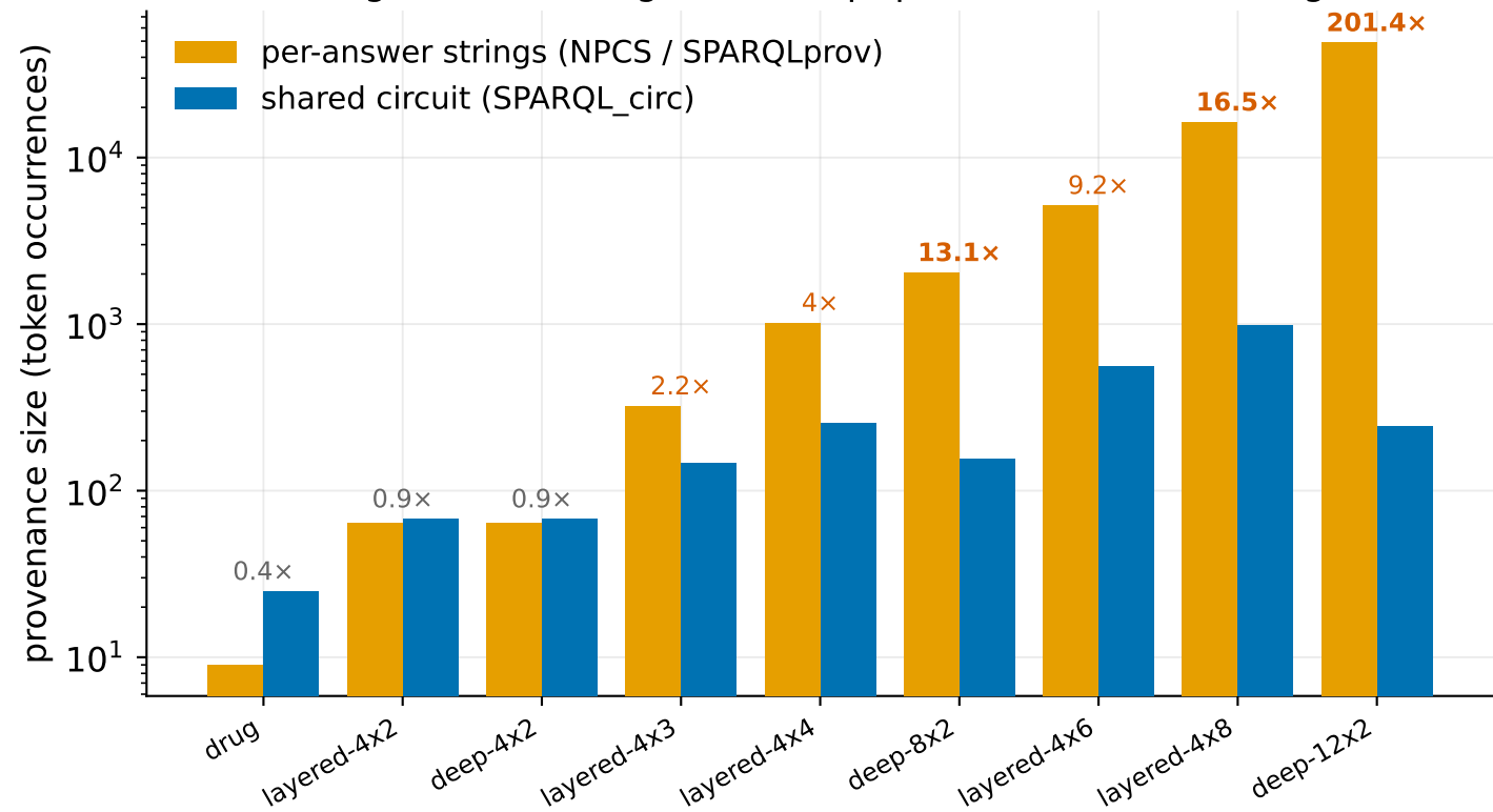
E2 Compactness: shared circuit vs. per-answer strings ( \times = string/circuit sharing ratio; deep queries \rightarrow orders of magnitude)
