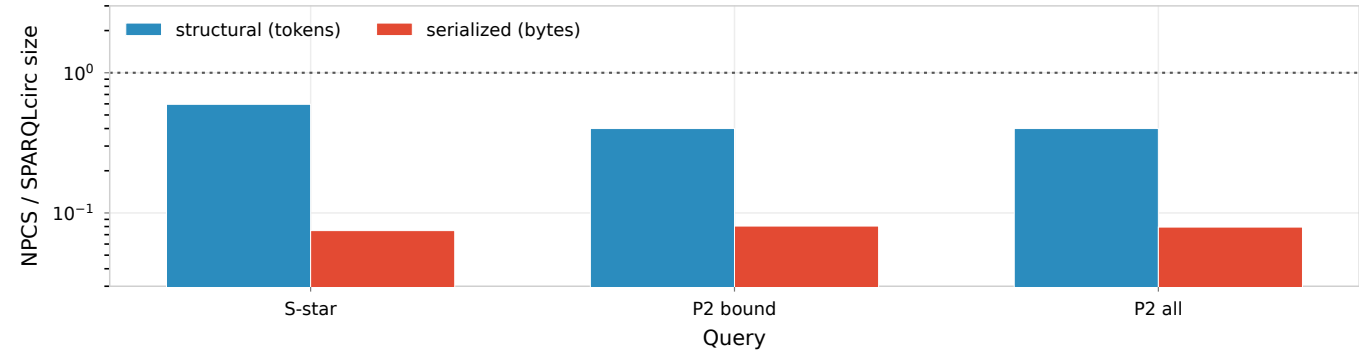
Representation size on low-sharing queries (ratio < 1 → SPARQLcirc larger)
