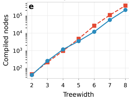
Growing treewidth: size
