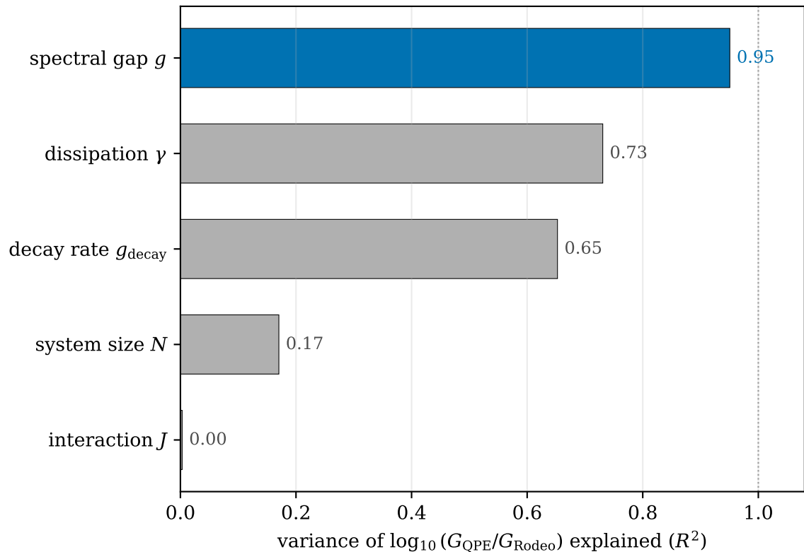
(b) the separation is the controlling variable
