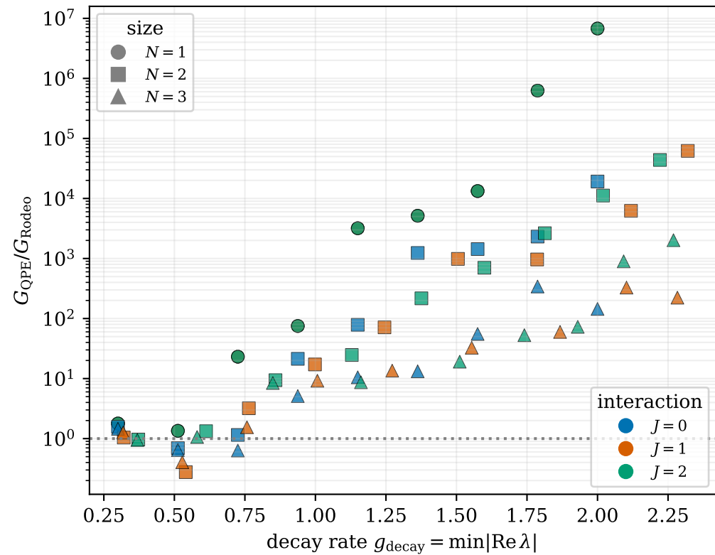
(a) vs decay rate: scatters, N -branches
