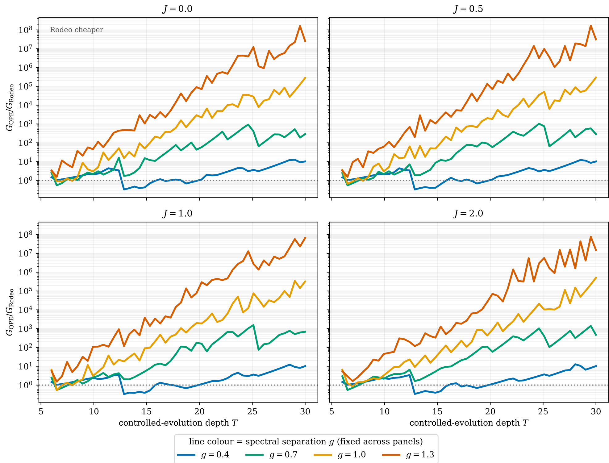
Larger separation g deepens the Rodeo advantage at each interaction strength J (TFIM, N = 2 )
