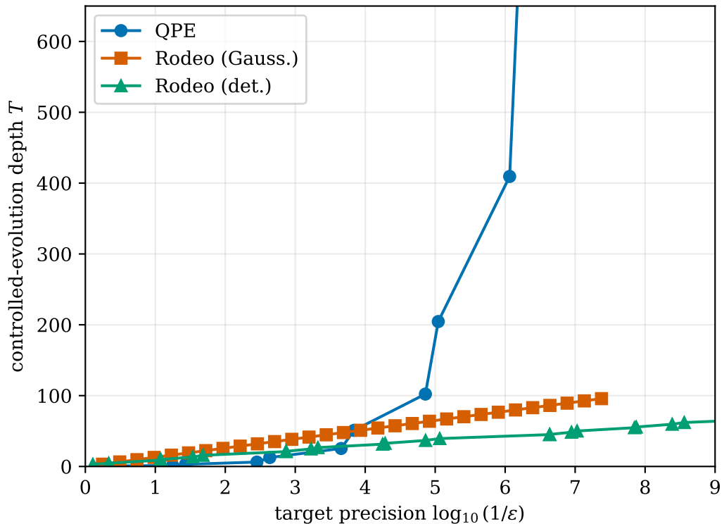
(b) linear: QPE diverges, Rodeo linear
