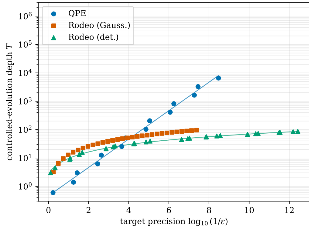
(a) semi-log: QPE power law vs Rodeo log
