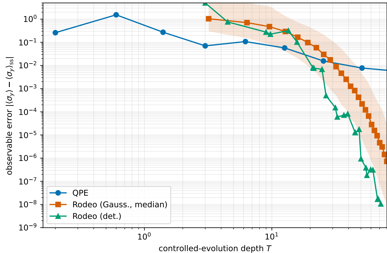
observable error vs depth ( h = 0.5 )
