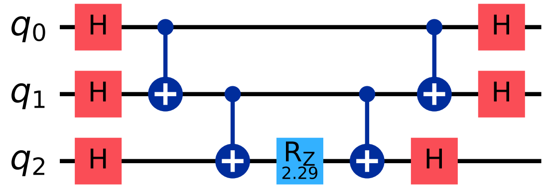
(b) one term \exp(-i \theta_{XXX} . XXX) : basis change, CNOT ladder, Rz, uncompute
