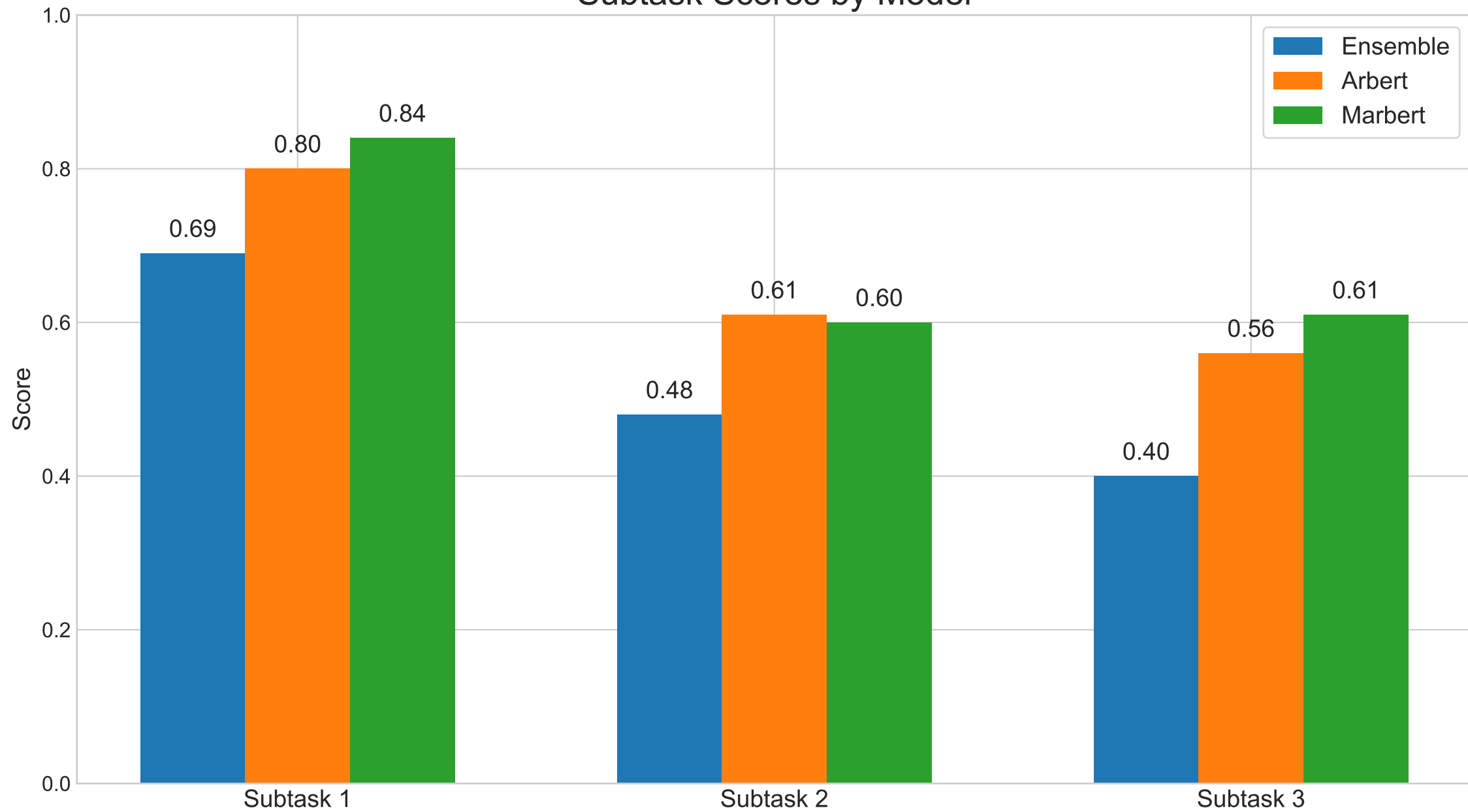
Subtask Scores by Model
