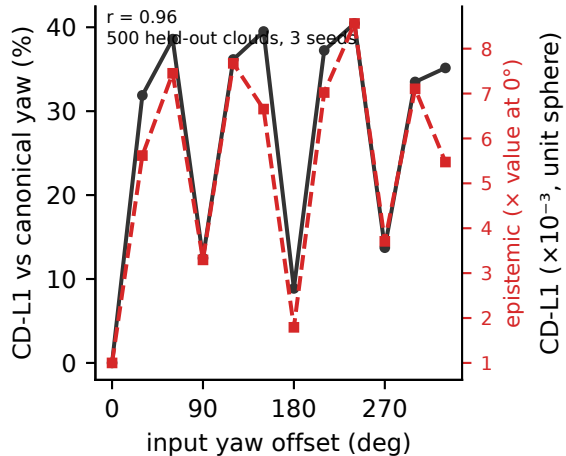
(a) yaw offset: CD and epistemic
