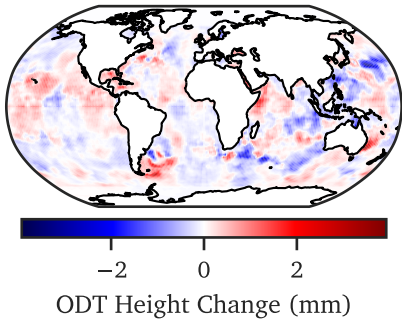
e) True Ocean Height Change
