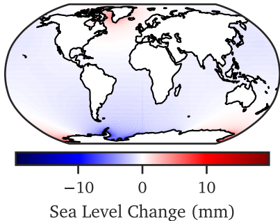
g) True Sea-Level Change
