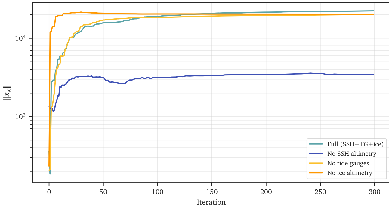
CG Convergence by Inversion Variant
