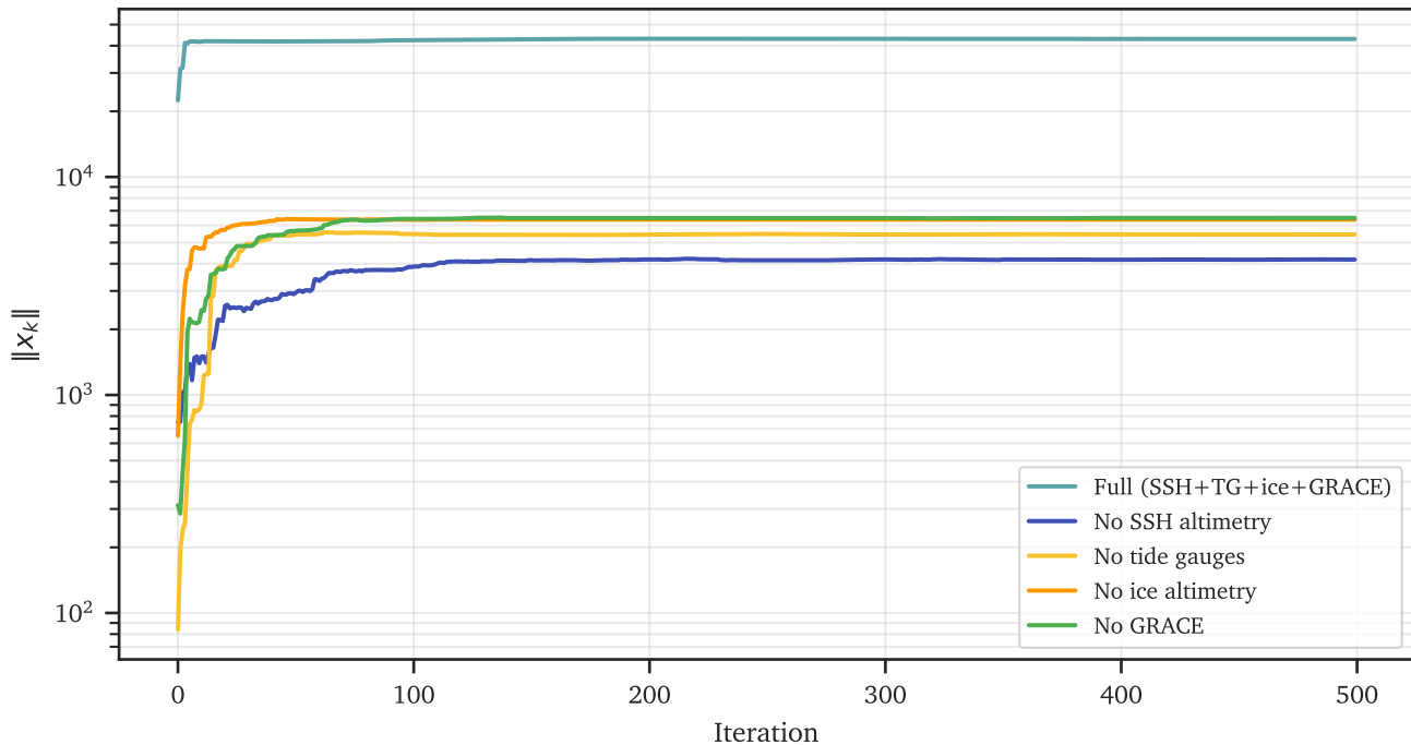
CG Convergence by Inversion Variant (with GRACE)
