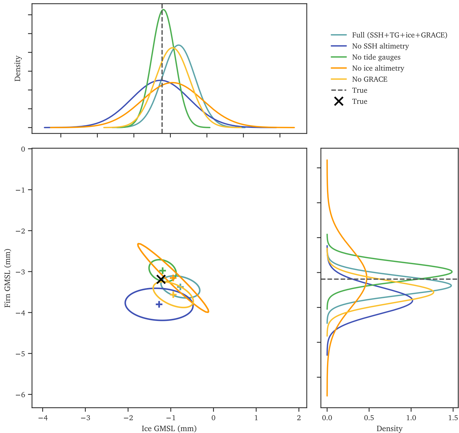
Knockout Sensitivity: Ice vs Firn GMSL (1-sigma ellipses, all variants)
