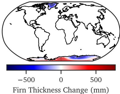
c) True Firn Thickness Change
