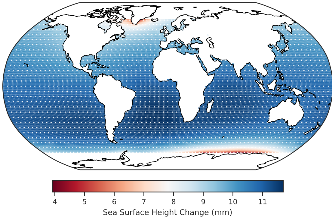
SSH sample with ocean-altimetry grid (5° spacing, 1402 points)
