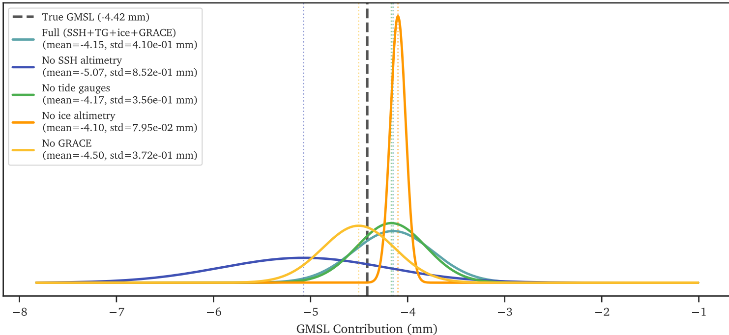
Knockout Test: GMSL Posterior Distributions (with GRACE)
