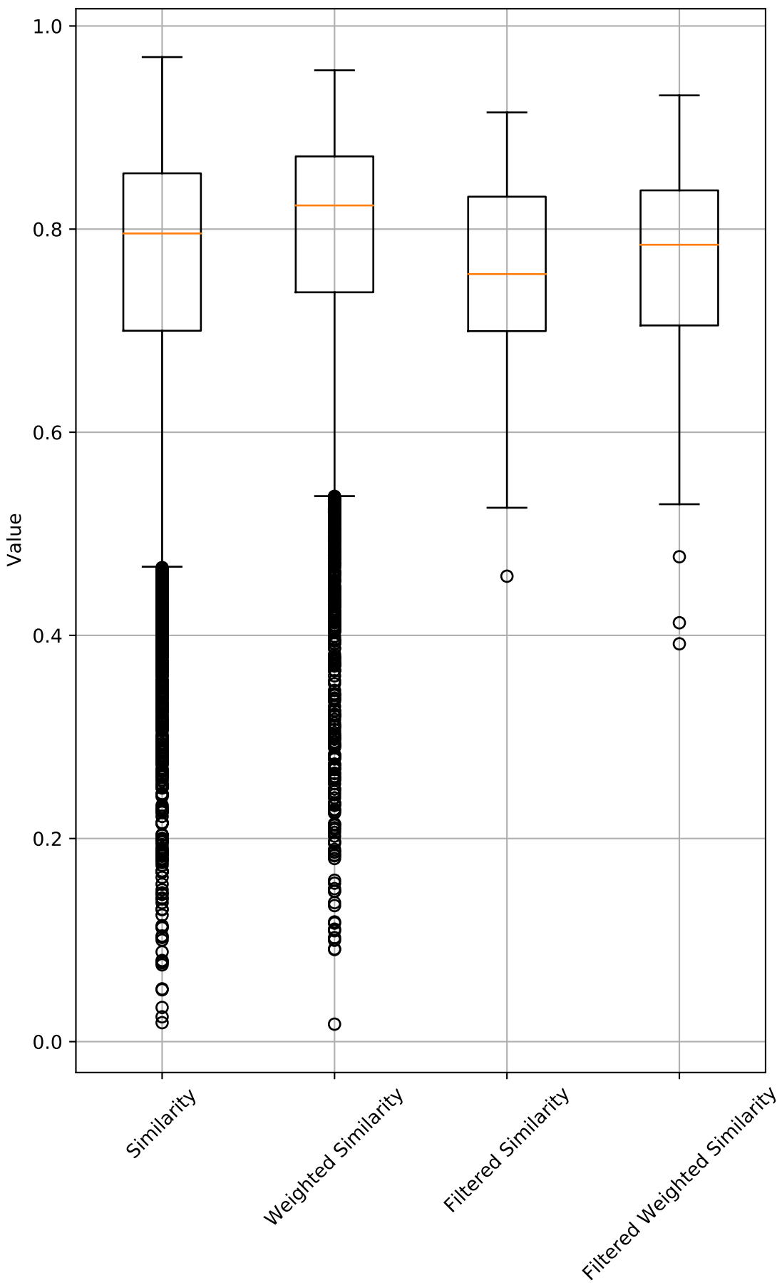
Boxplot of Similarity and Weighted Similarity with and without Fluoro Ratio Filter
