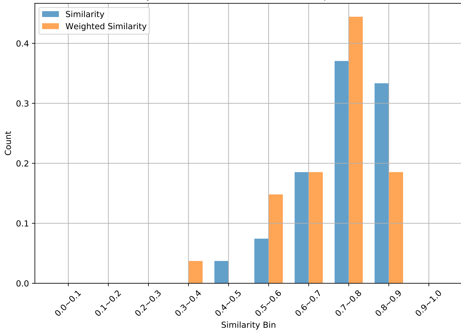
Similarity Distribution (bin width = 0.1, sample size = 27)
