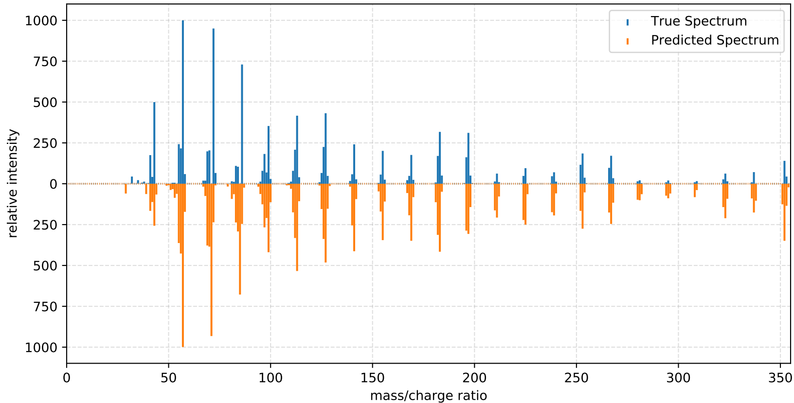
Record 1 Comparison Cosine: 0.7253 | Weighted: 0.9046
