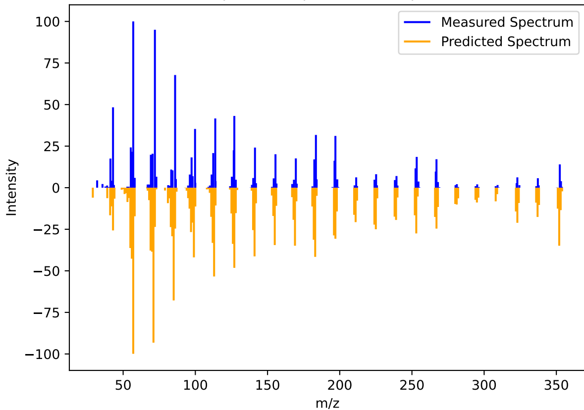
Compound 1 Spectrum Comparison
