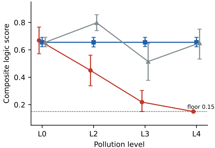
Llama-3.1-8B-Instruct (INT4)
