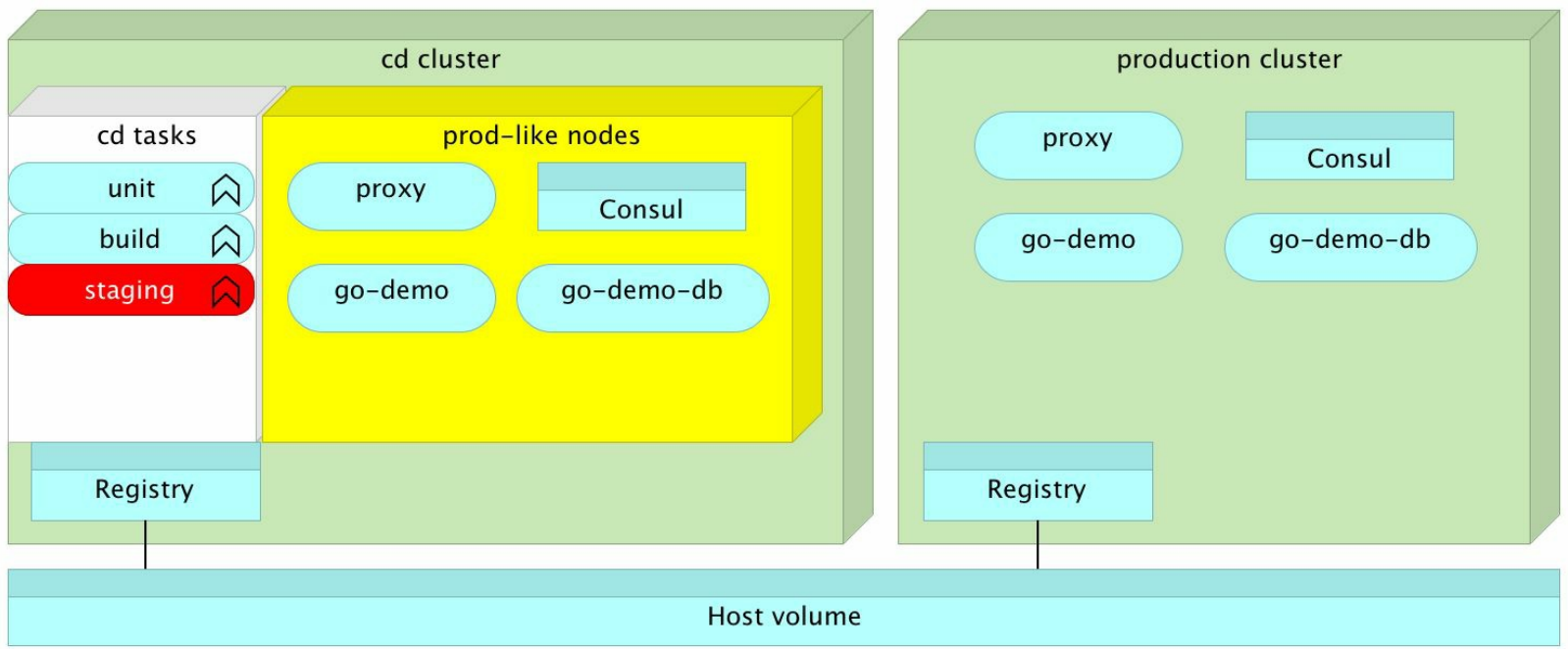
Figure 5-7: Staging or functional tests run inside the swarm-test-1 node
