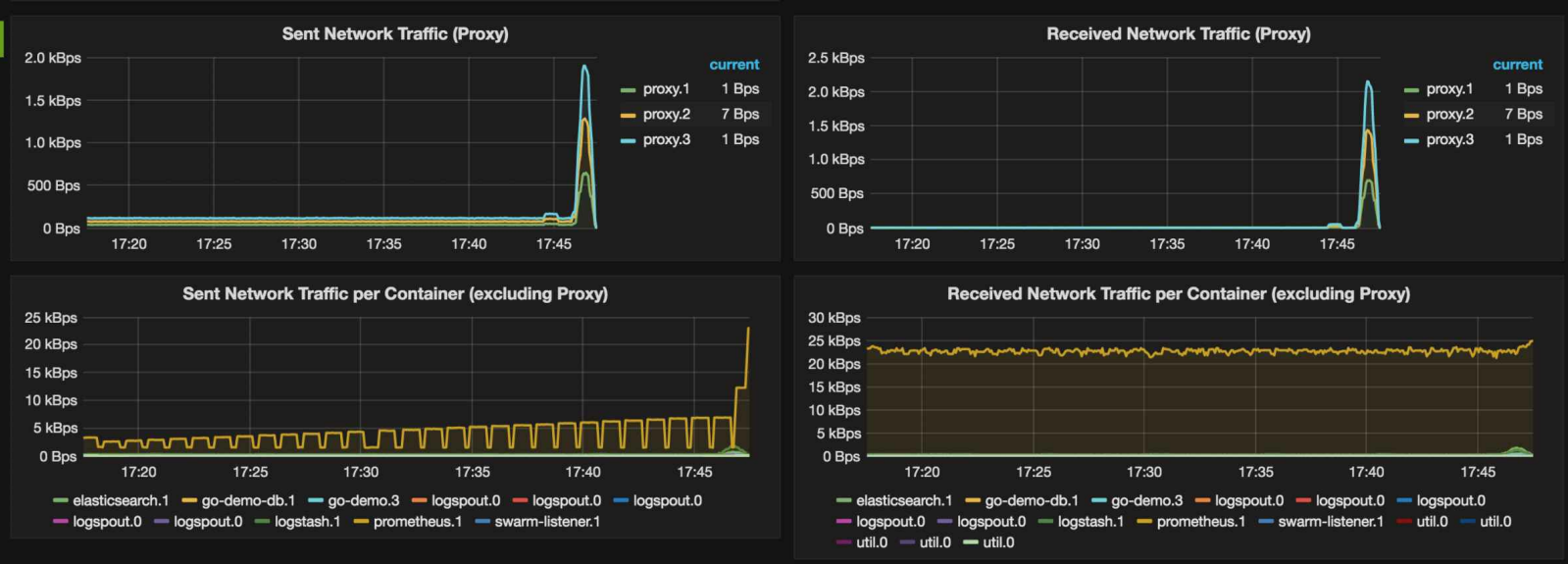
Figure 9-10: Grafana dashboard with network traffic graphs
