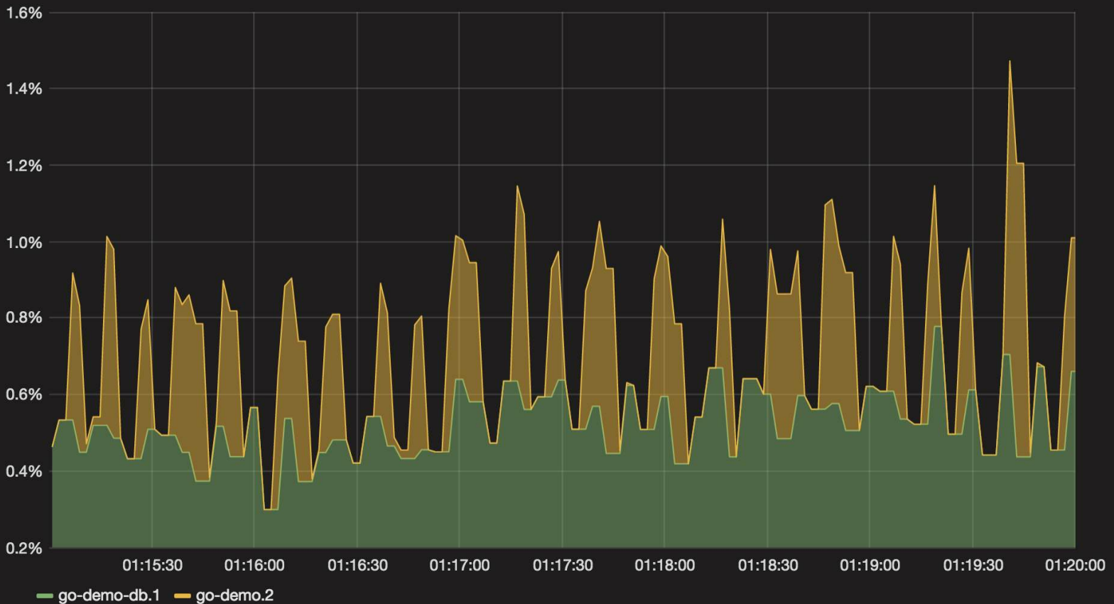
Figure 9-9: Grafana graph with CPU Usage per Container filtered by Service Group
