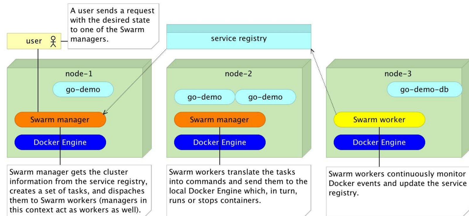
Figure 4-6: Docker Swarm (standalone) flow
