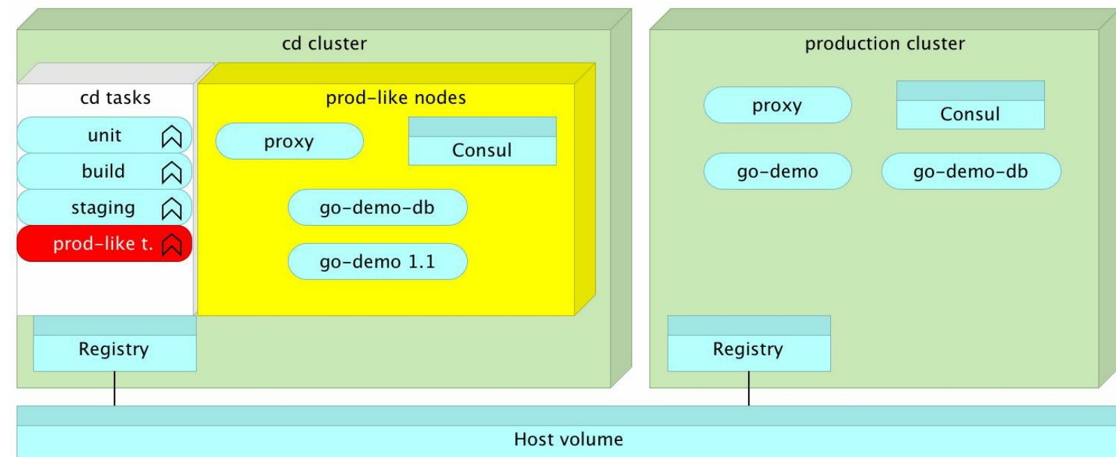
Figure 5-9: Production tests are run against the updated service inside the CD cluster
