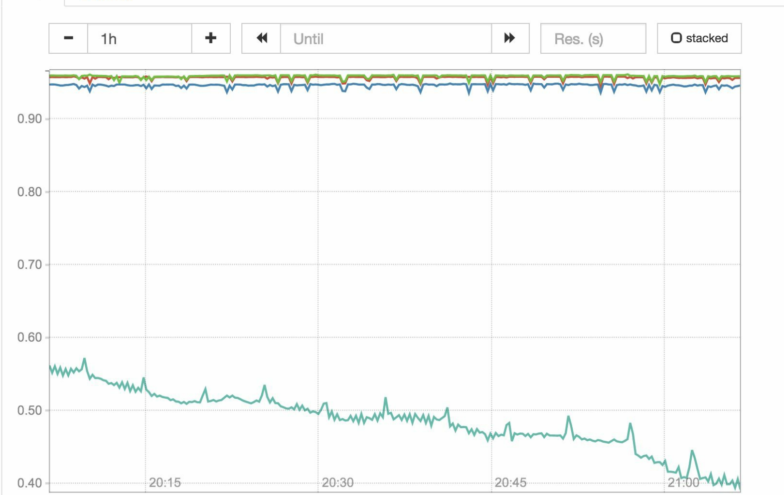
Figure 9-4: Prometheus graph with CPU idle rate
