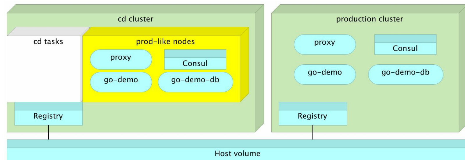
Figure 5-4: CD and production clusters with services
