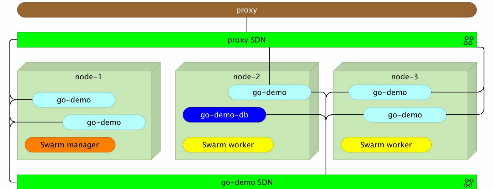
Figure 3-5: Docker Swarm cluster with the go-demo service scaled
