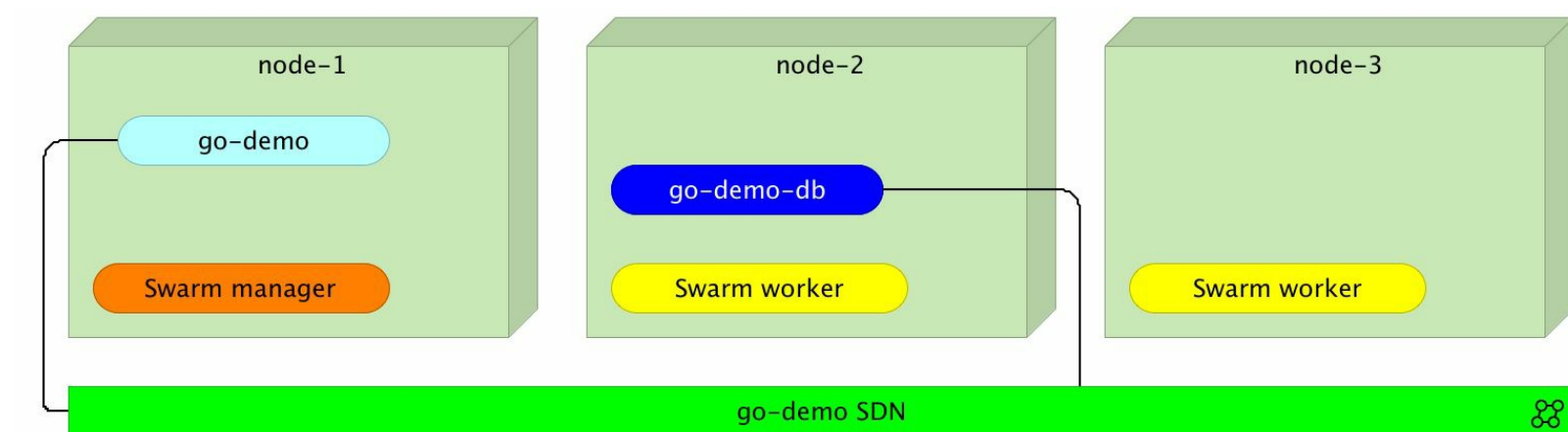
Figure 2-8: Docker Swarm cluster containers communicating through the go-demo SDN
