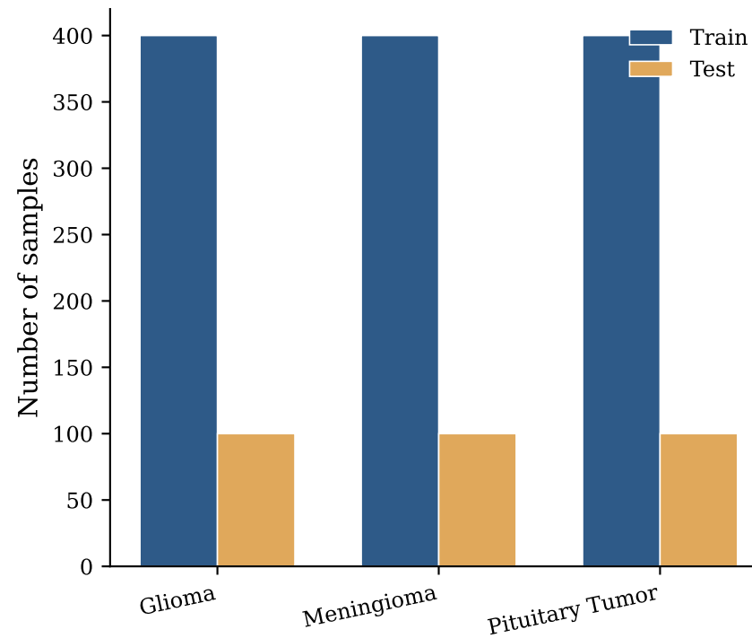
Class distribution
