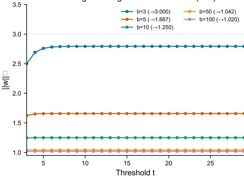
Convergence of geometric norm to b/(b-2)
