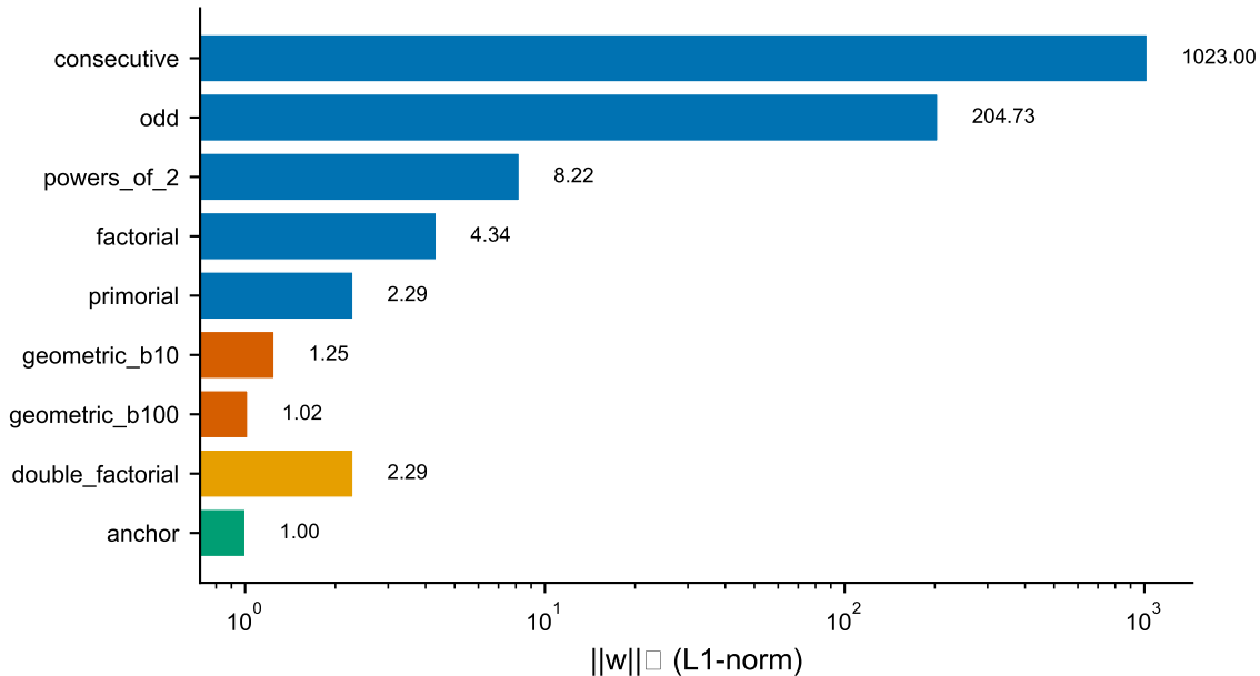
Lagrange weight norm by evaluation point family (t=10)
